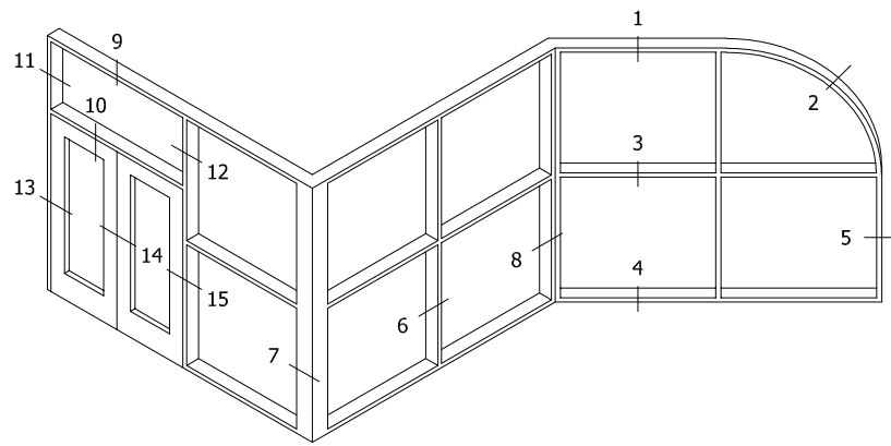
TYPICAL ELEVATION
