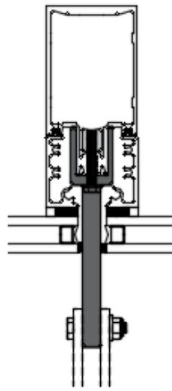
P6942 - 400CW/T Intermediate Mullions
