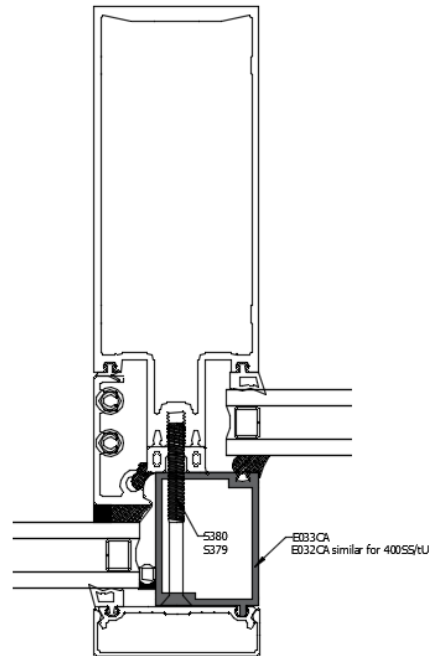
New detail allows for transition from cassette to captured curtain wall. Available for 400CW/T, 400SS & 400TU
