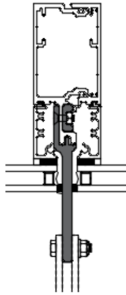
P6944 / P6945 - 400SS Intermediate Mullions
