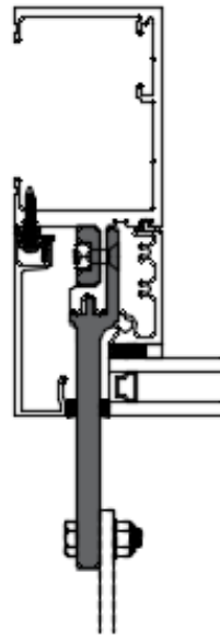
P6944 / P6945 - 400SS Vertical End Jamb
