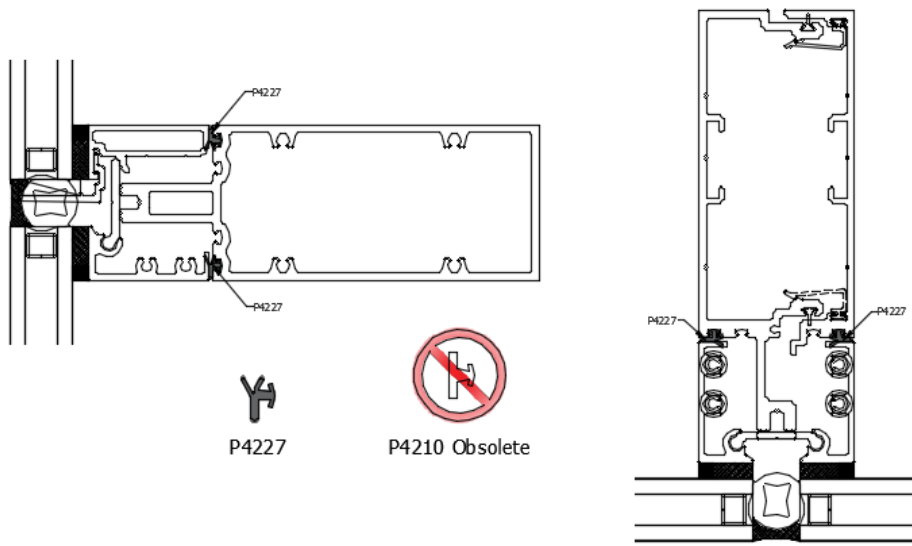
New cassette backer gasket P4227 (replaces P4210)
