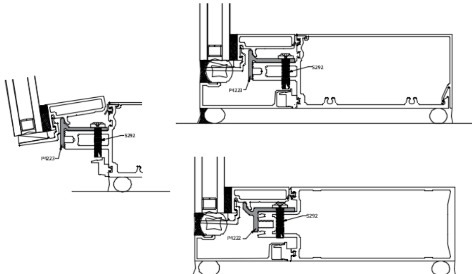
New base roll-over sill anchor clip for 400CW/T, 400SS & 400TU
