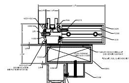
9B STANDARD TRANSOM
