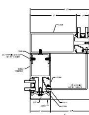
7 OUTSIDE CORNER STANDARD
