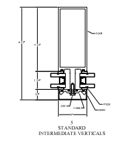
5 STANDARD INTERMEDIATE VERTICALS
