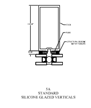
5A STANDARD SILICONE GLAZED VERTICALS
