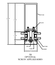
5B OPTIONAL SCREW-APPLIED HORN
