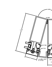
7C 90 INSIDE CORNER - SSG STANDARD
