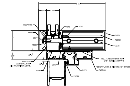
9 STANDARD TRANSOM
