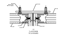
13 T-ANCHOR STANDARD
