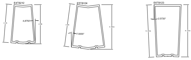
SPLAYED MULLION
