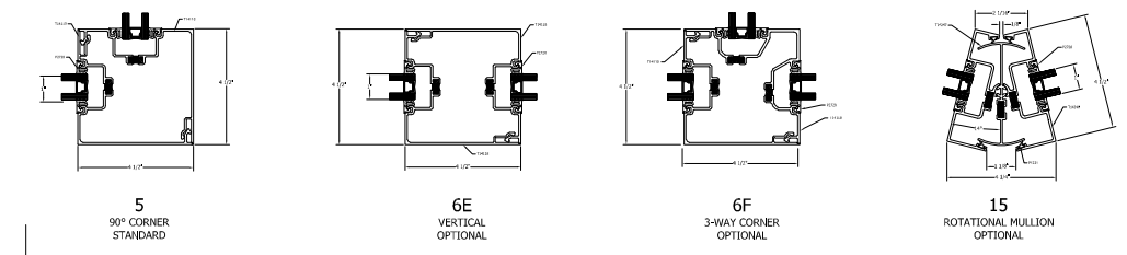
CORNER & WIDE PROFILE OPTIONS NOTE: ABOVE OPTIONS ONLY AVAILABLE AS SINGLE POUR & DEBRIDGE
